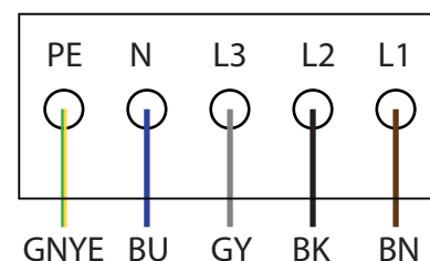
Figure 7: Bornes de raccordement CA
