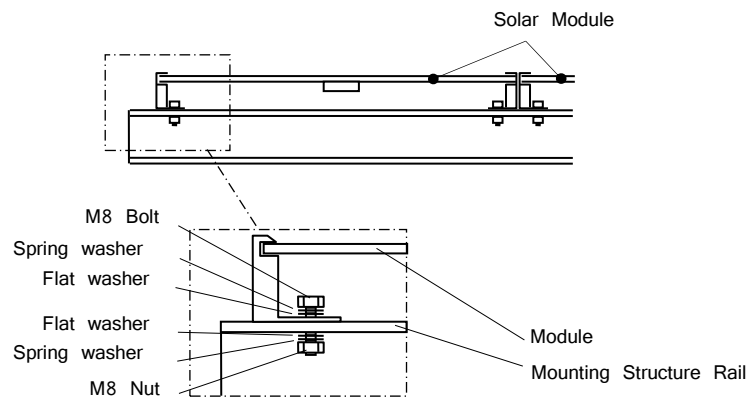
Figure 10-2 Installation B
