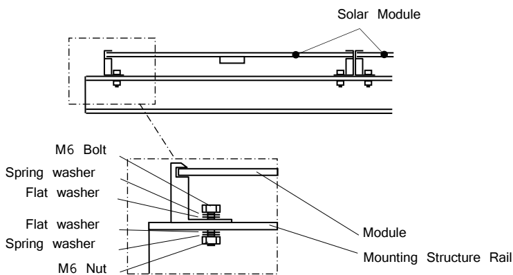
Figure 2-2 Installation B
