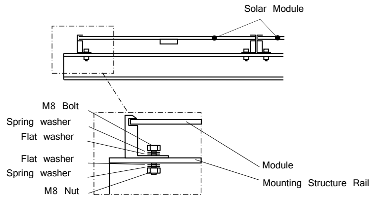
Figure 8-2 Installation B
