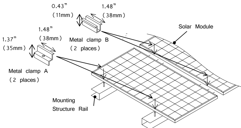
Figure 2-1 Installation A
