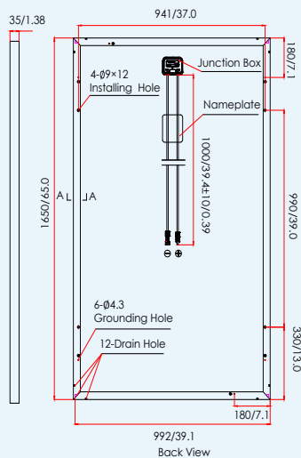
DIMENSIONS OF PV MODULE
